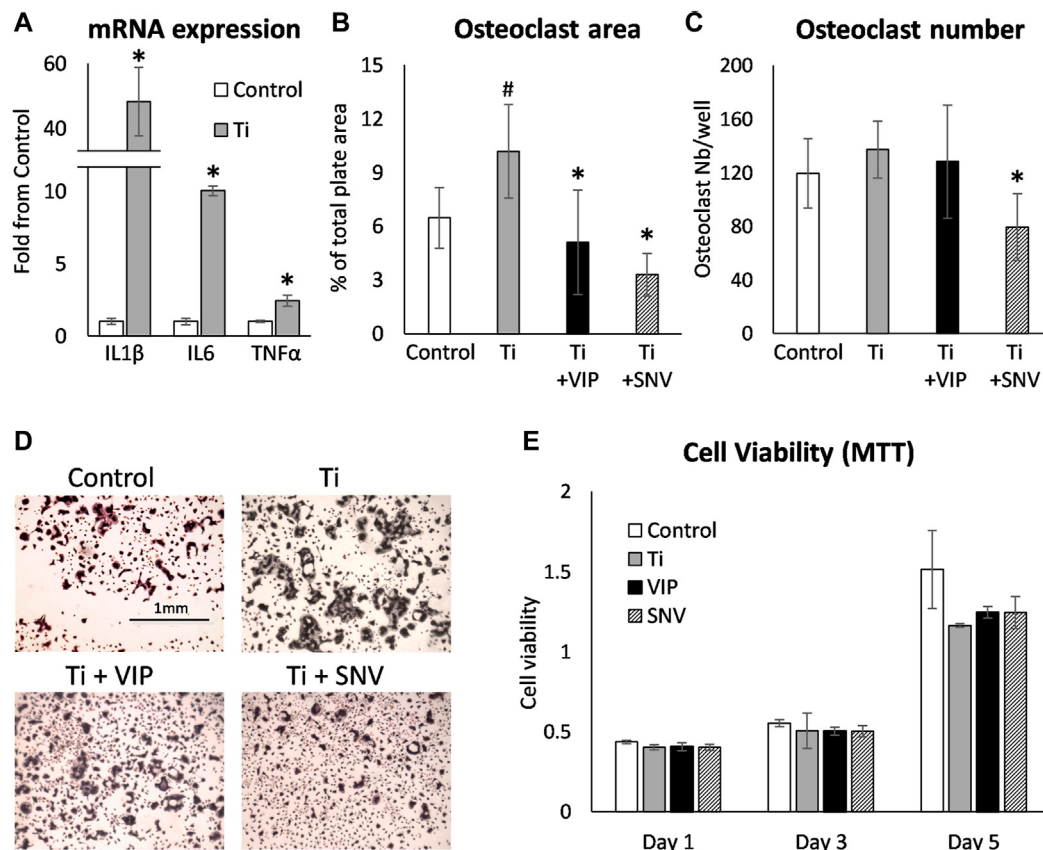
FIGURE 4 | VIP and SNV alleviate the osteoclastogenic effect of TiP-induced inflammation. (A) Primary BMDM were exposed to TiP and RNA was collected after 24 h. mRNA expression is presented as Mean \pm SD fold change versus Control. * p <0.05 vs. Control. (B–D) Primary murine preosteoclasts were cultured in 20 ng/ml M-CSF and 50 ng/ml RANKL for 48 h. Conditioned medium from macrophages (Control) and macrophages exposed to Ti particles (Ti, as in A) was then added together with 10^{-6} M of VIP or SNV (or saline) for 48 h before TRAP staining. Data are Mean \pm SD for osteoclast % surface area (B) and number per well (C). (D) Representative images all acquired at a 4x original magnification. The scale bar for all images is in the upper left panel. n=8 , # p <0.05 vs. Control; * p <0.05 vs. Ti, ANOVA. (E) Primary murine macrophages/preosteoclasts were cultured in 20 ng/ml M-CSF and Ti particles, 10^{-6} M of VIP or SNV, or saline only. MTT viability assay was performed after 1, 3 and 5 days and presented as optical density values. N=5 , no statistical differences were found between the treatment groups. Data are Mean \pm SD in arbitrary OD units.
